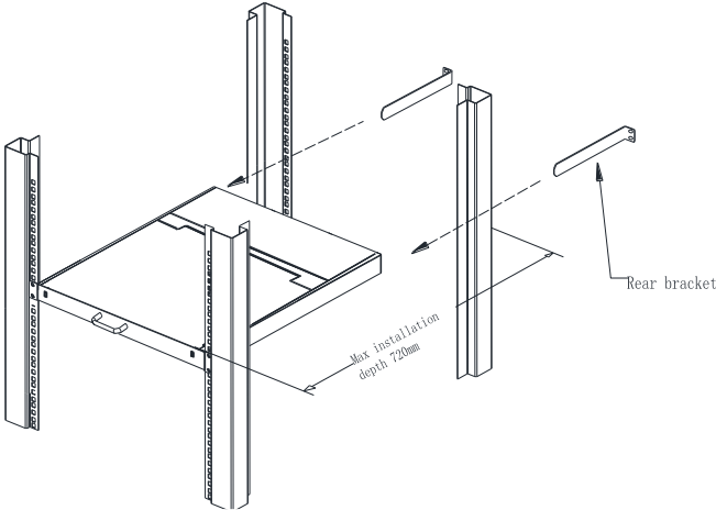
1-2.1 rack mounting (1)
