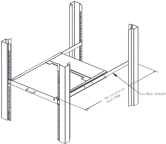
1-2.2 rack mounting (2)
